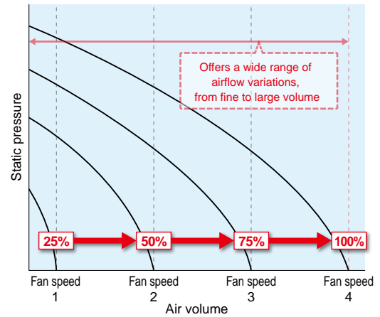
■ New model characteristic curves
